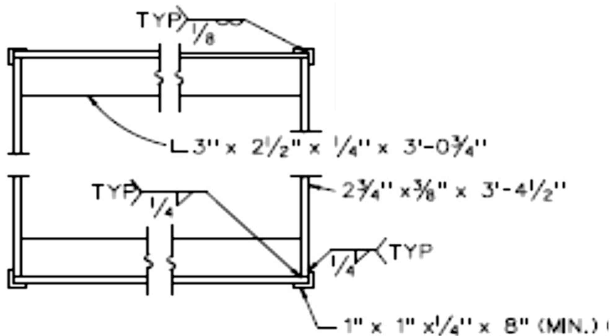
DETAIL OF FRAME
